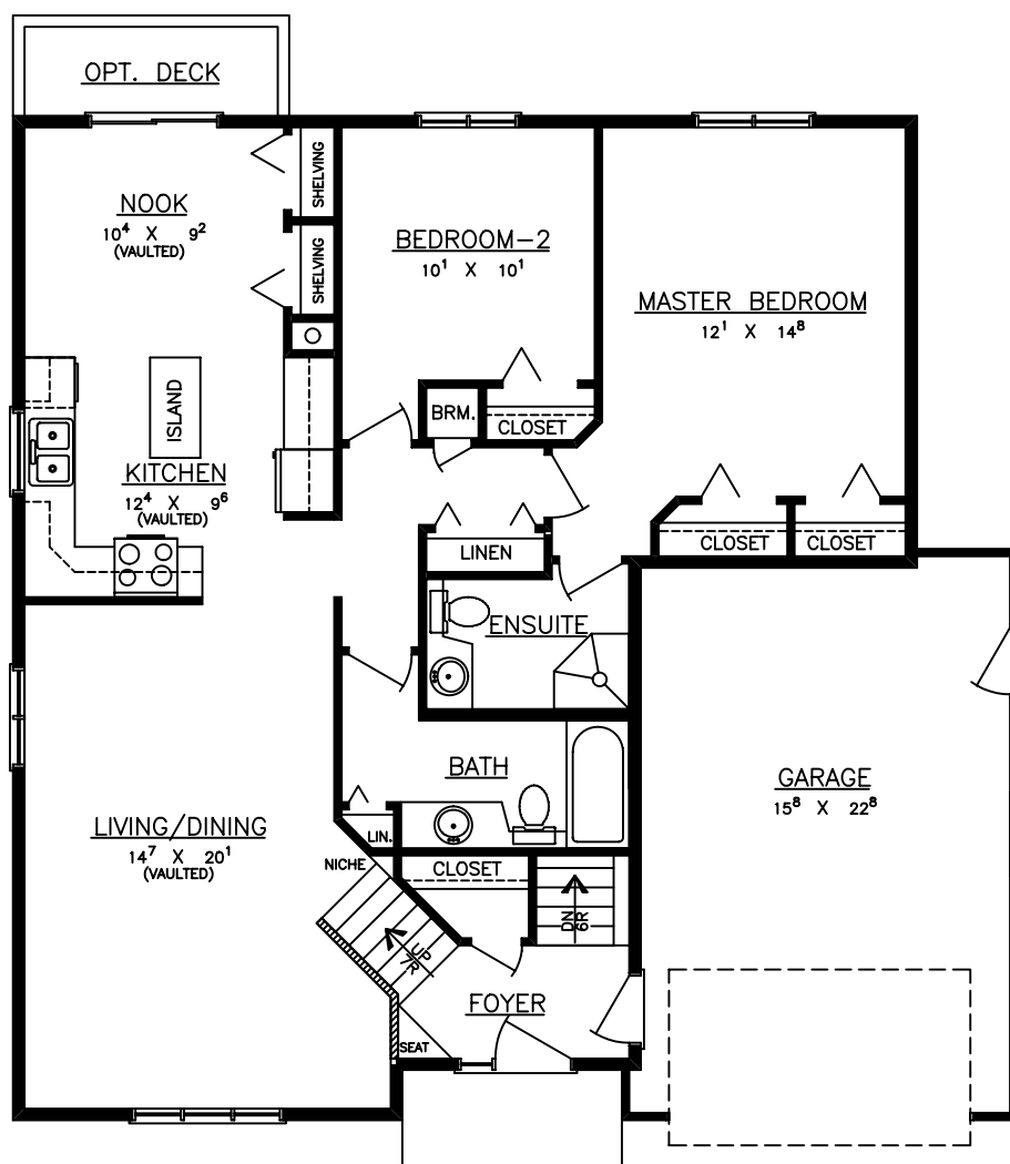
FLOOR PLAN
